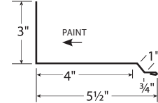
UNIVERSAL SIDEWALL SF1 - Girth 9.25"
