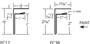
F CHANNEL FC12 - Girth 7.5" FC38 - Girth 7.375"
