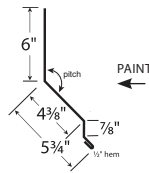
UNIVERSAL ENDWALL EF - Girth 12.5"
