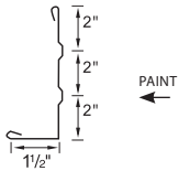
BEADED FASCIA BFT9(color)102 - Girth 8.25"
