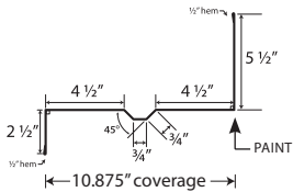
GABLE BASE SOFFIT GB1 - Girth 20.25"
