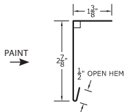
SOFFIT F ADAPTOR SFA - Girth 4.75"
