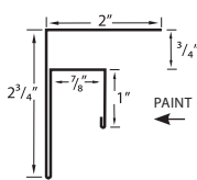
PANEL-LOC PLUS F&J PFJ - Girth 9.125"
