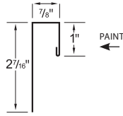
J-TRIM JT - Girth 4.8125"
