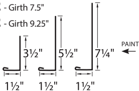
SOFFIT F ADAPTOR SFA - Girth 4.75"
