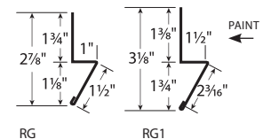
RAT GUARD RG - Girth 4.75" RG1 - Girth 5.5625"
